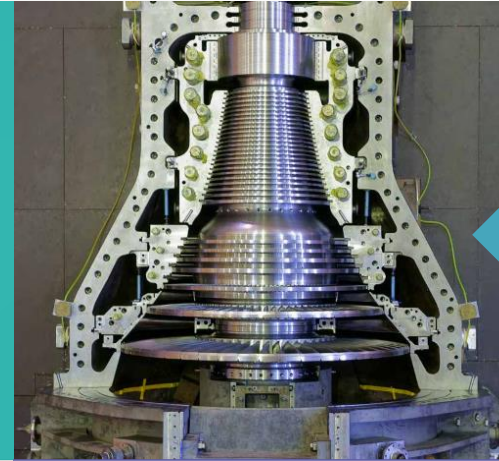
Steam Turbine MST-50C
